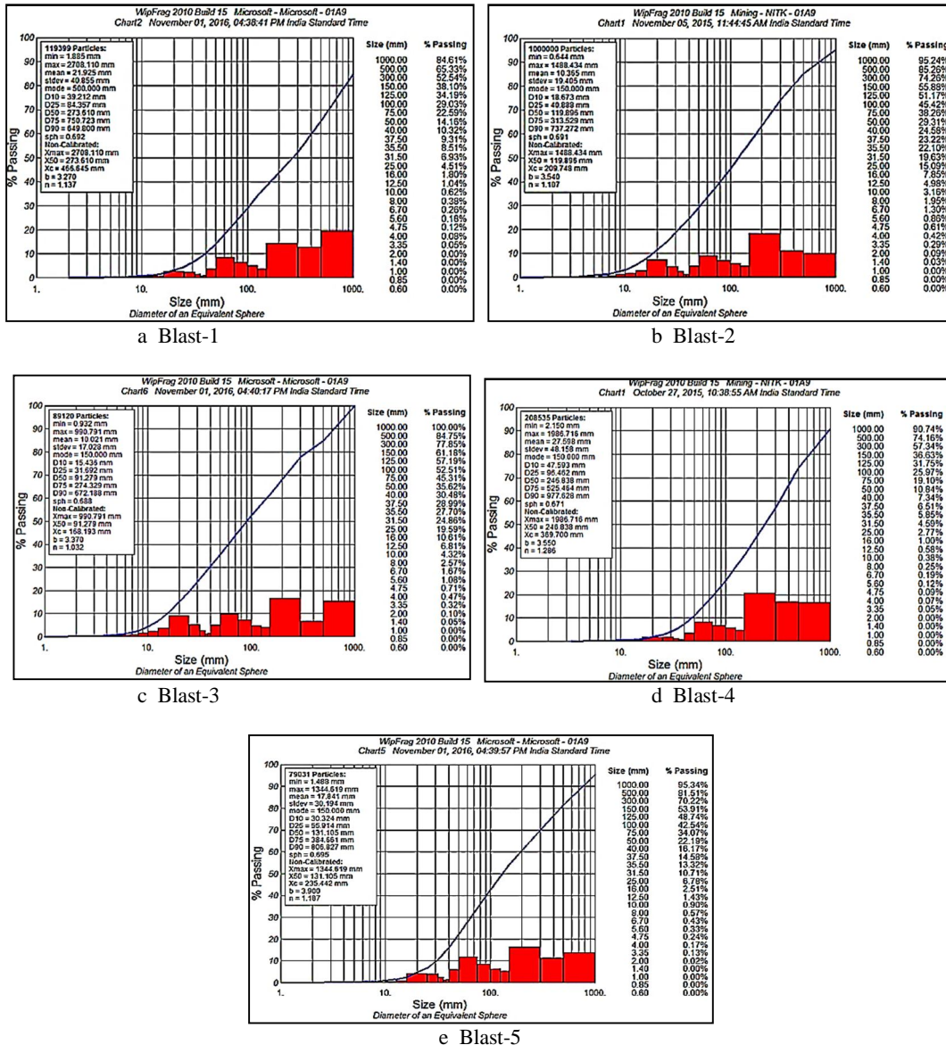
Figure 9. Fragmentation analysis of different blasts at Mine-B
